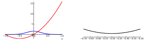
Figure 1: At left, \pi(a | s) for a Gaussian policy at a given state (blue) and \nabla_{\mu} \log \pi(a | s)Q(a, s) for Q = \frac{1}{2} + \frac{1}{2}a (red). At right, the variance of a simple single-sample Monte Carlo estimator as a function of the baseline. In a simple multi-sample Monte Carlo method, the variance would go down as the square root of the number of samples.
