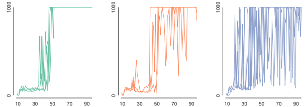
Figure 3: Three runs for EPG (left), DPG (middle) and SPG (right) for the InvertedPendulum-v1 domain, demonstrating that EPG shows much less unlearning.
